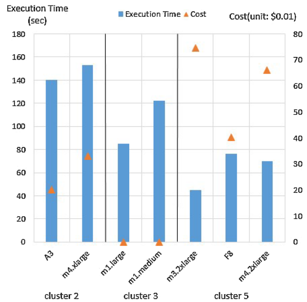
Fig. 1 Execution time and cost comparison of clusters, reflecting CFD application characteristics
