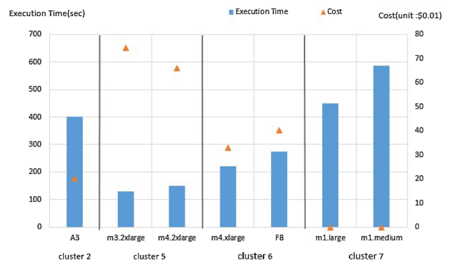
Fig. 2 Execution time and cost comparison of clusters, reflecting Montage application characteristics
